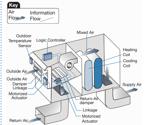
Fig. 4: The Components of an Economizer (Source: E Source Cooling Atlas)
